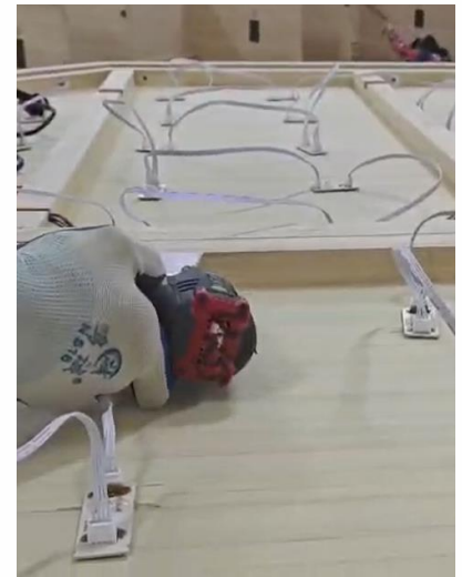
15. Screw the ceiling panels together and along the edges
